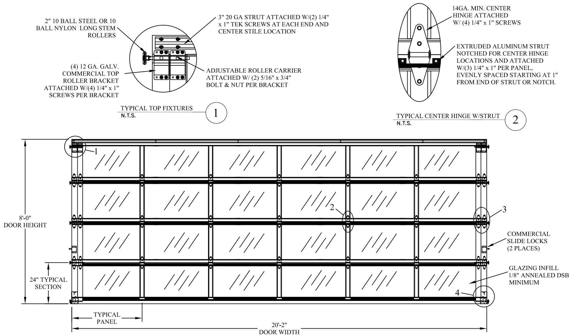
DOOR INTERIOR ELEVATION
